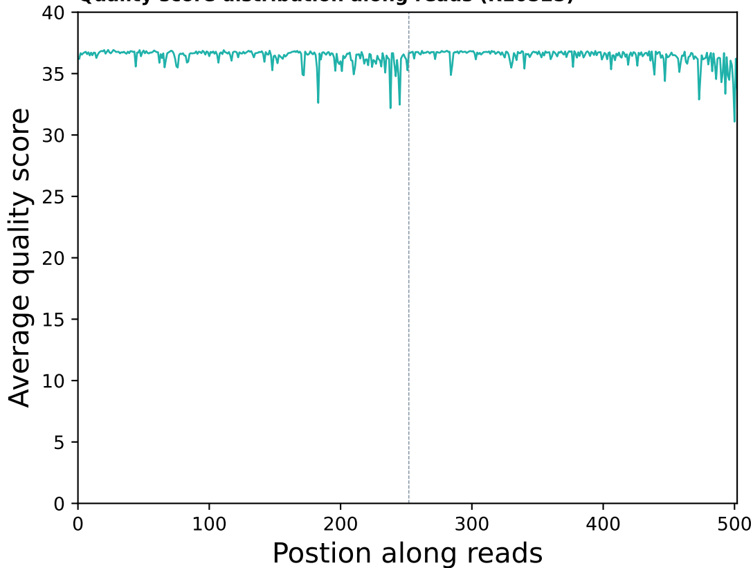
Quality score distribution along reads (R10525)
